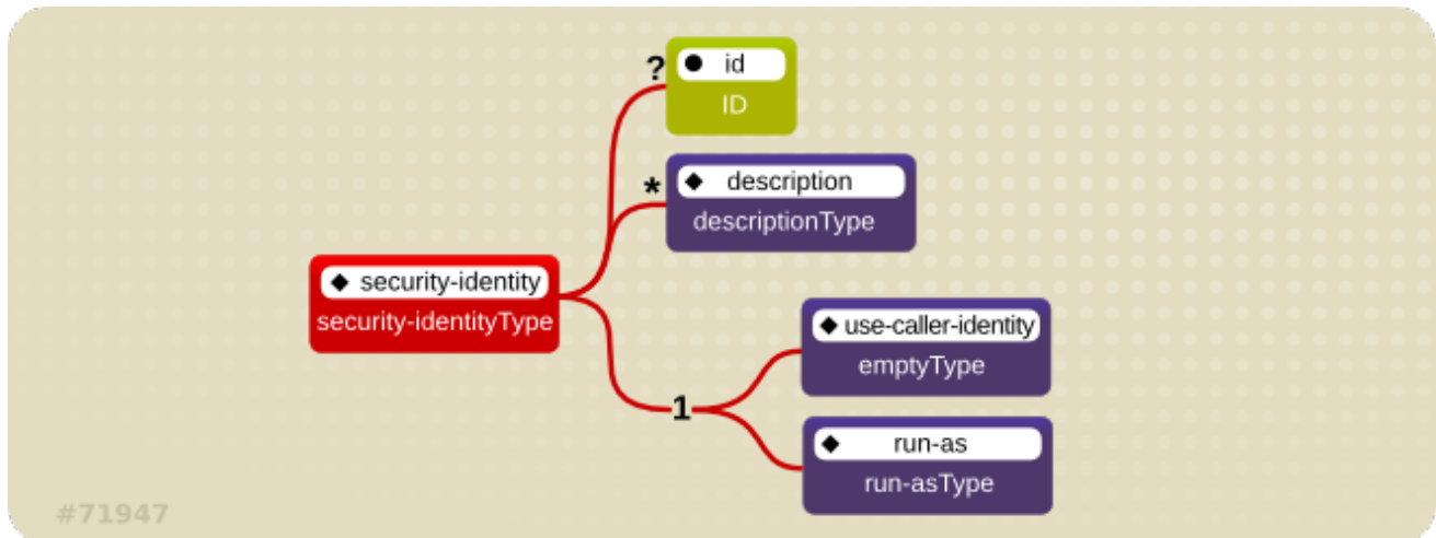
Figure 8.2. Java EE Security Identity Data Model
